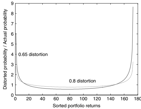
Figure 3. Ratio of distorted to actual probabilities in Anticipated Utility, w(P) = \frac{p^c}{[p^c+(1-p)^c]^{1/c}} . This figure shows the ratio of distorted to actual probability in Anticipated Utility (Section 5.3) with w(P) = \frac{p^c}{[p^c+(1-p)^c]^{1/c}} for c = 0.65 and c = 0.8 .
